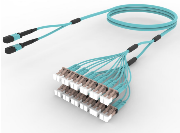
OM3 MPO (Female) to LC, InstaPATCH® 360 Ruggedized Fanout Cable, 24-Fiber, Low Smoke Zero Halogen
